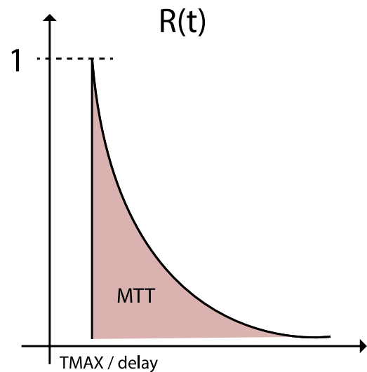
Figure 1: residual function over time
