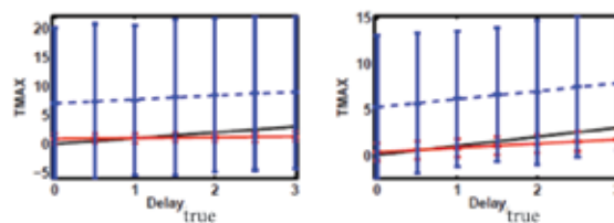
Figure 5: true delay vs estimated Tmax Parameter validated on CT phantom data. Blue: oSVD / Red: BDM Originally published in IEEE 26
