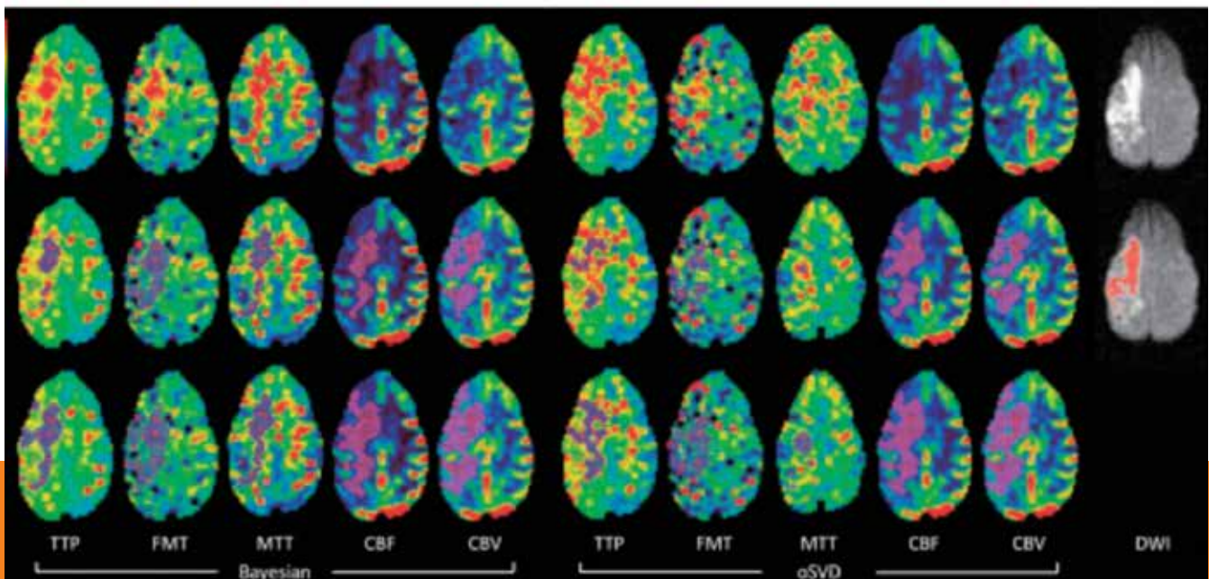
Figure 7: perfusion maps from Bayesian-based deconvolution method and oSVD algorithms. Various perfusion maps and DWI map are shown in the top row. The area of the final infarct is shown in purple (time to peak [TTP], first moment of transit [FMT], and mean transit time [MTT] maps) or pink (cerebral blood flow [CBF] and cerebral blood volume [CBV]) at the best threshold, which was determined with the final infarct of the specimen volume (middle row) and DWI volume (bottom row). The volumes of the final infarct differ among maps and algorithms. In this particular subject, perfusion abnormalities in the FMT, MTT, and CBF of the Bayesian-based deconvolution methods correspond well to the high signal area of DWI. Originally published in Magn Reson Med Sci 30
